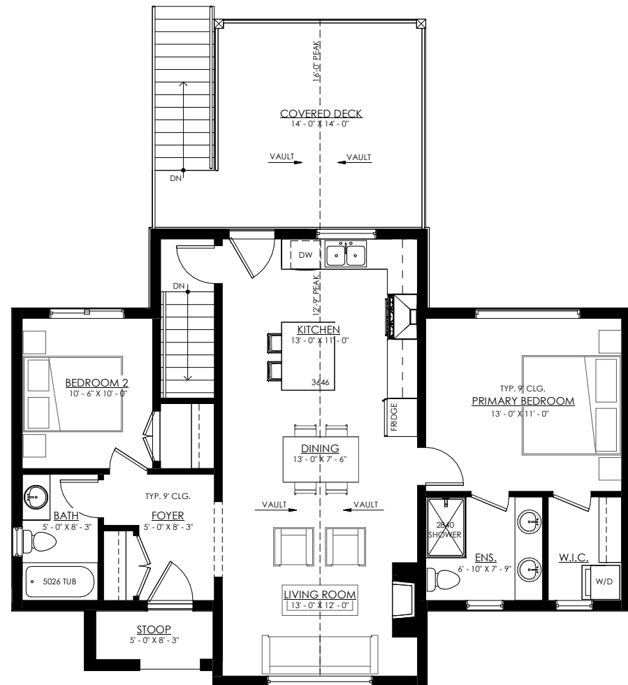
MAIN FLOOR MAIN FLOOR AREA 970 SF
